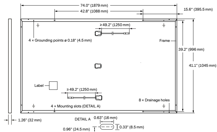
Fig. 2: External dimensions (in inch (mm)) and components for Q.PEAK DUO ML-G10.2 and Q.PEAK DUO ML-G10.4
