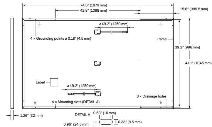
Fig. 1: External dimensions (in inch (mm)) and components for Q.PEAK DUO ML-G10, Q.PEAK DUO ML-G10+, Q.PEAK DUO BLK ML-G10, Q.PEAK DUO BLK ML-G10+, Q.PEAK DUO ML-G10.a, Q.PEAK DUO ML-G10.a+, Q.PEAK DUO BLK ML-G10.a and Q.PEAK DUO BLK ML-G10.a+
